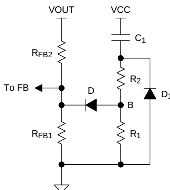
Figure 12. Soft-Start Circuit
